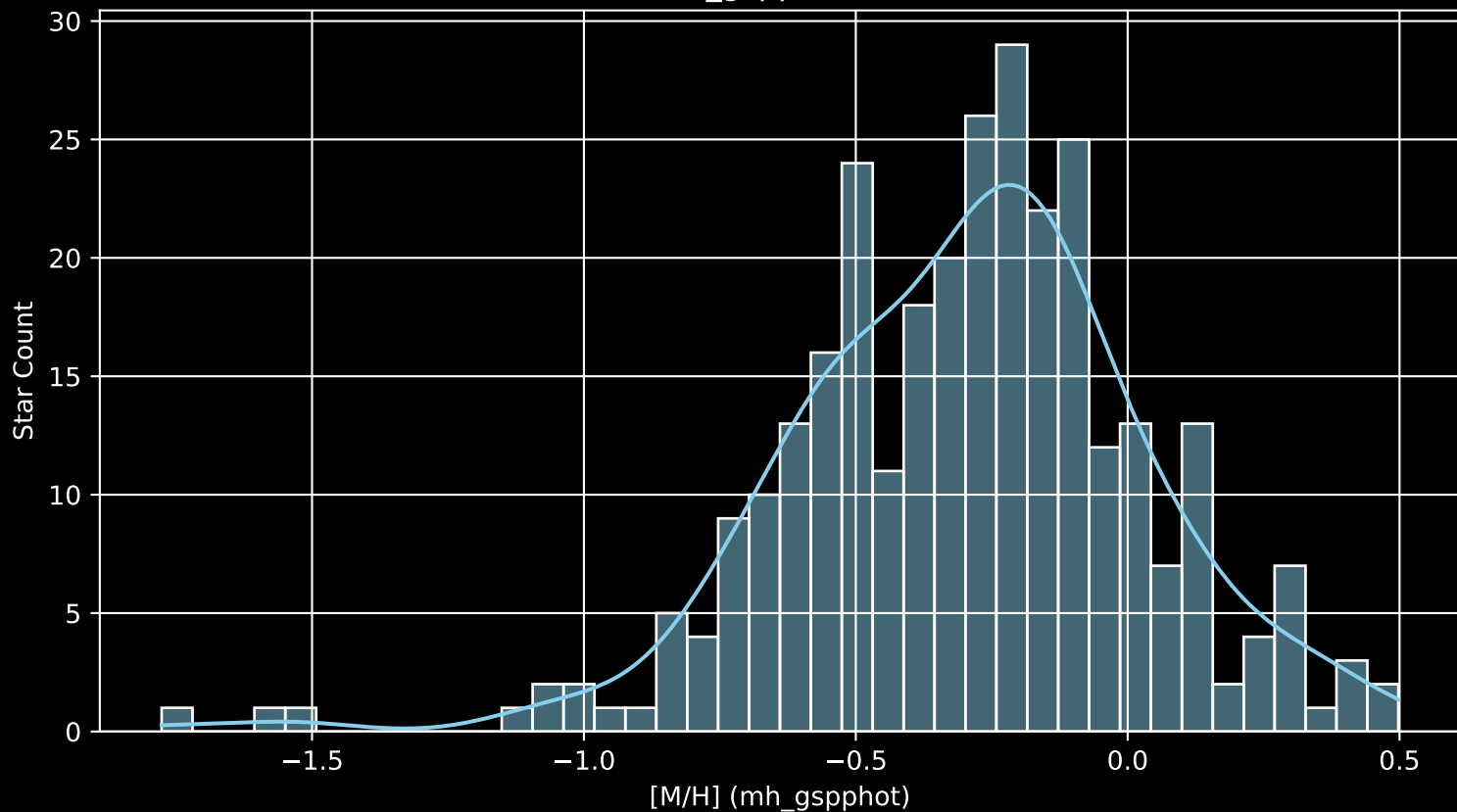
GALAH DR4 Field: [7042] [M/H] (mh_gspphot) (n= 306)
