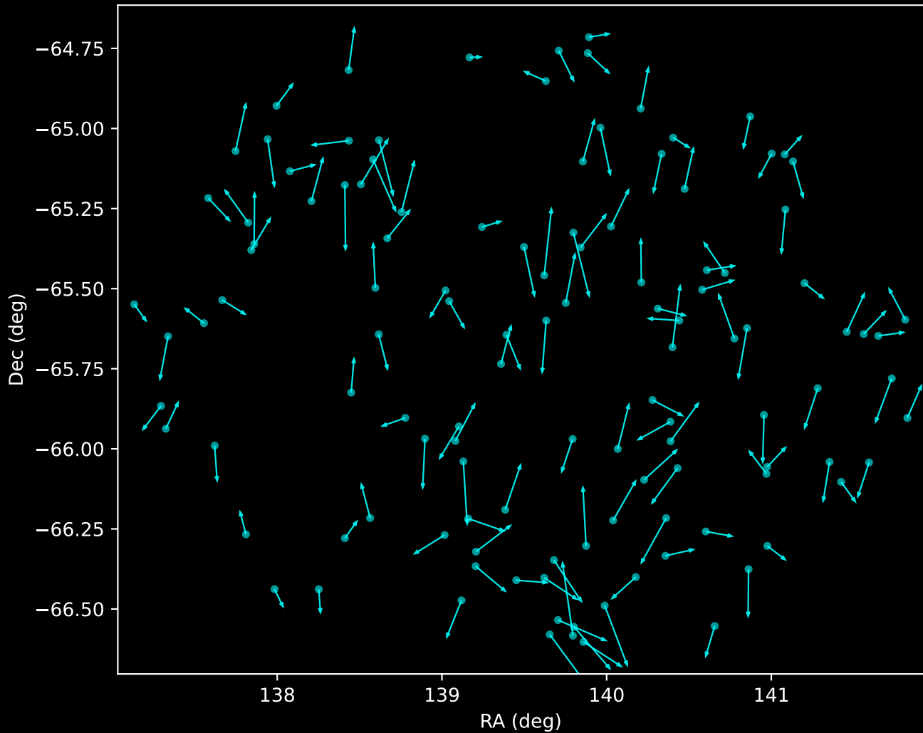
GALAH DR4 Noise Stream Proper Motion Vectors (n=119)
