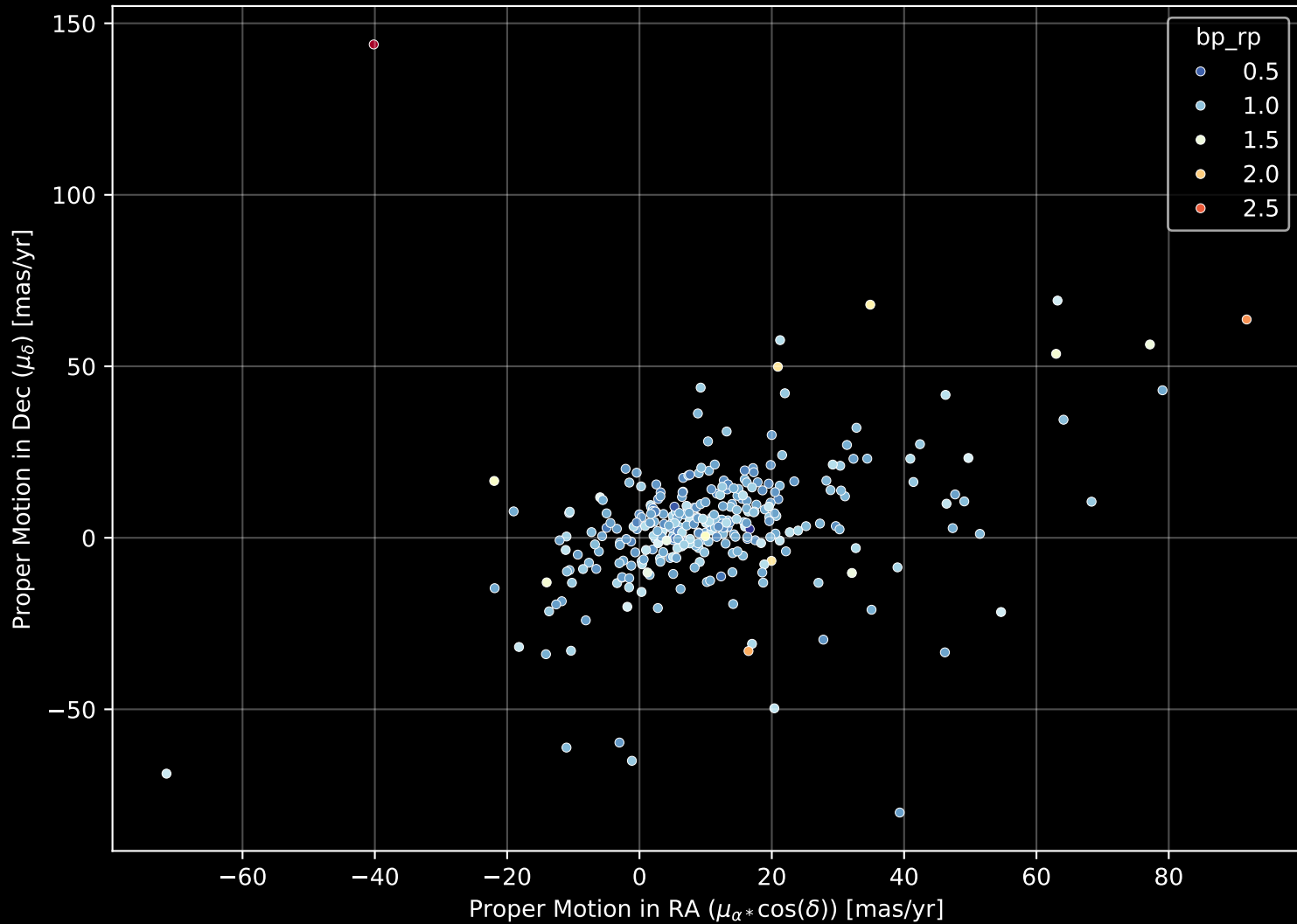
GALAH DR4 Field: [7042] Proper Motion Diagram (n= 311)
