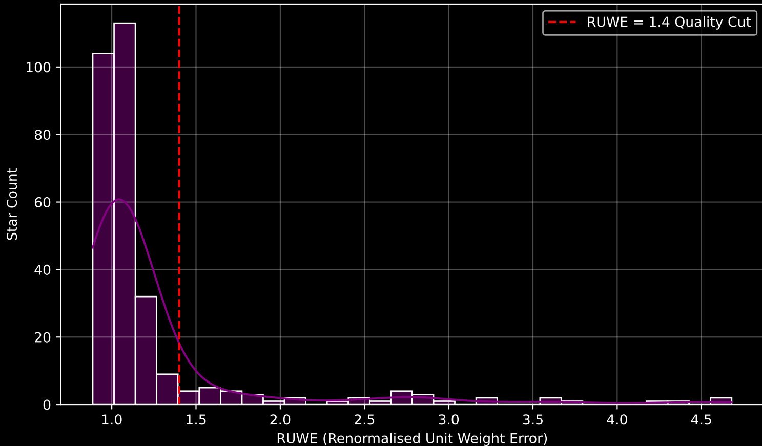
GALAH DR4 Field [7042] RUWE Distribution (n= 298)
