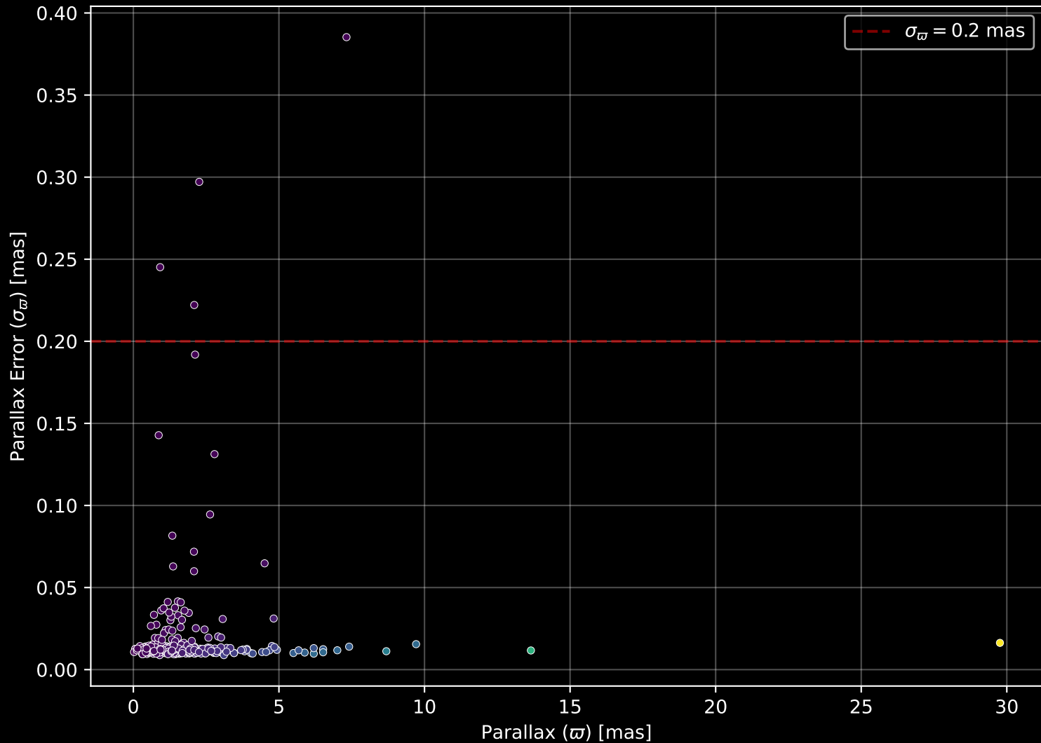
GALAH DR4 Field: [7042] Parallax Quality (n= 311)
