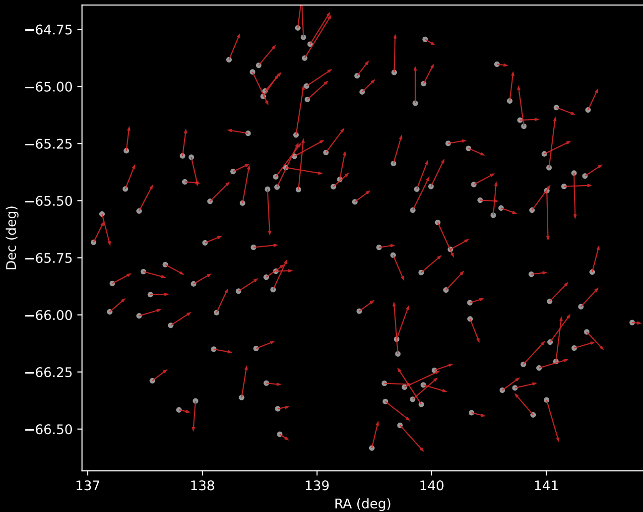
GALAH DR4 Cluster 6 Proper Motion Vectors (n=123)
