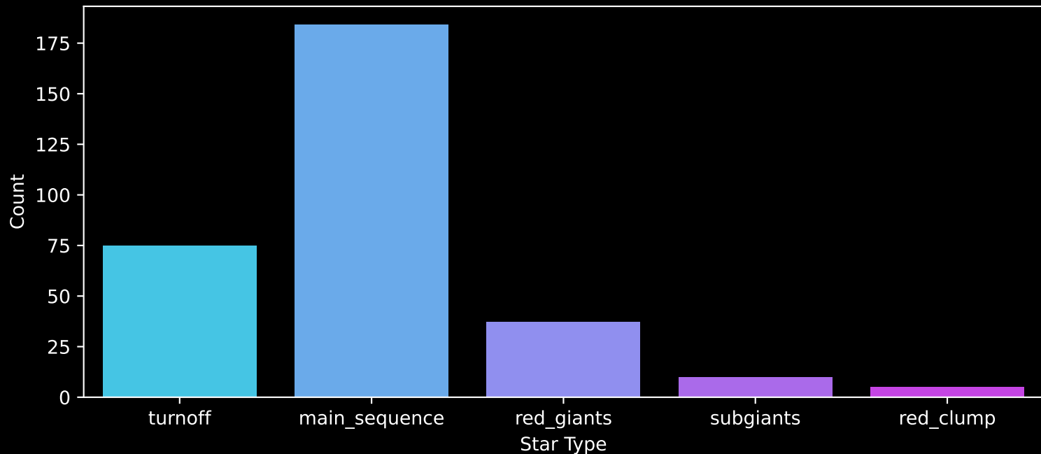
GALAH DR4 Field: [7042] Count plot of Star Type
