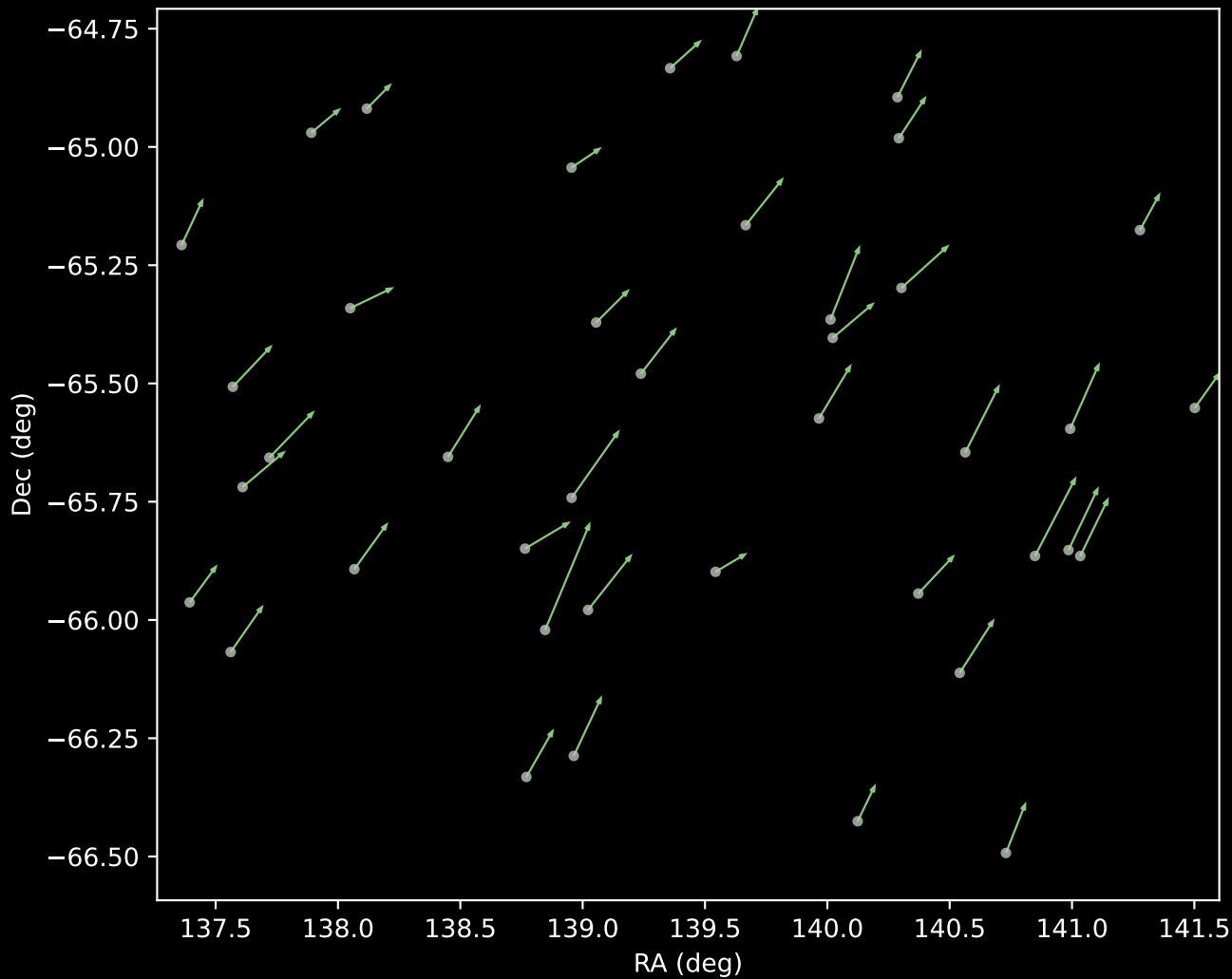
GALAH DR4 Cluster 5 Proper Motion Vectors (n=41)
